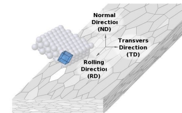
Cubic-structured crystallite in a deformed sample
