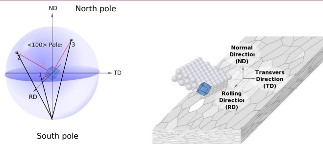
Lines between \langle 100 \rangle poles and south pole Intersection with equatorial plane
